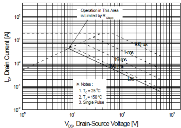
Figure 9-2. Maximum Safe Operating Area for JFFM5N60C
