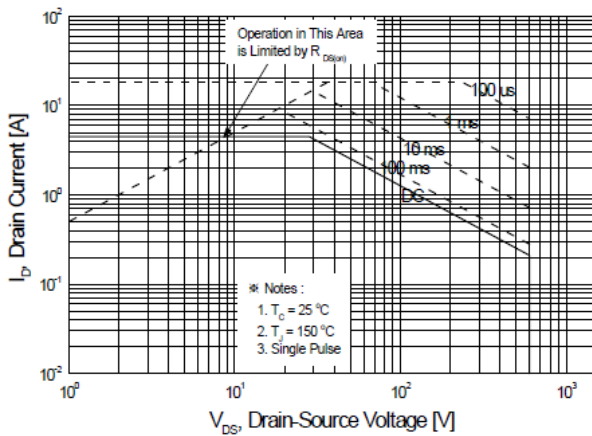
Figure 9-1. Maximum Safe Operating Area for JFPC5N60C
