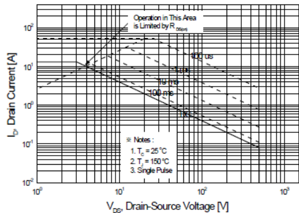
Figure 9-2. Maximum Safe Operating Area for JFFM13N50C
