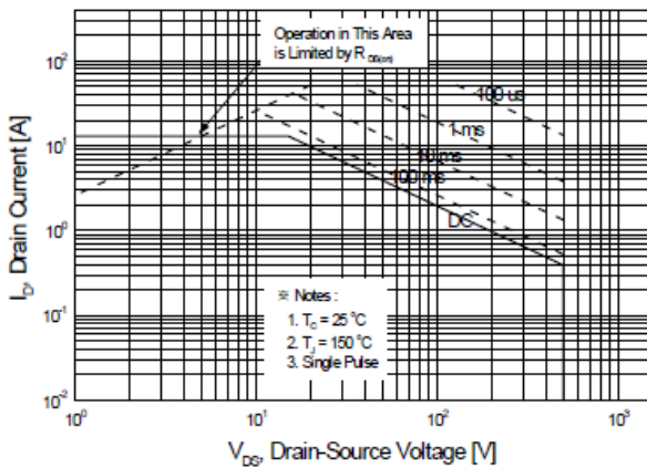
Figure 9-1. Maximum Safe Operating Area for JFPC13N50C
