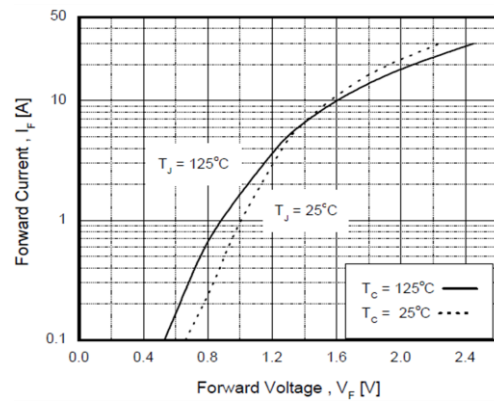
Figure 16. Forward Characteristics
