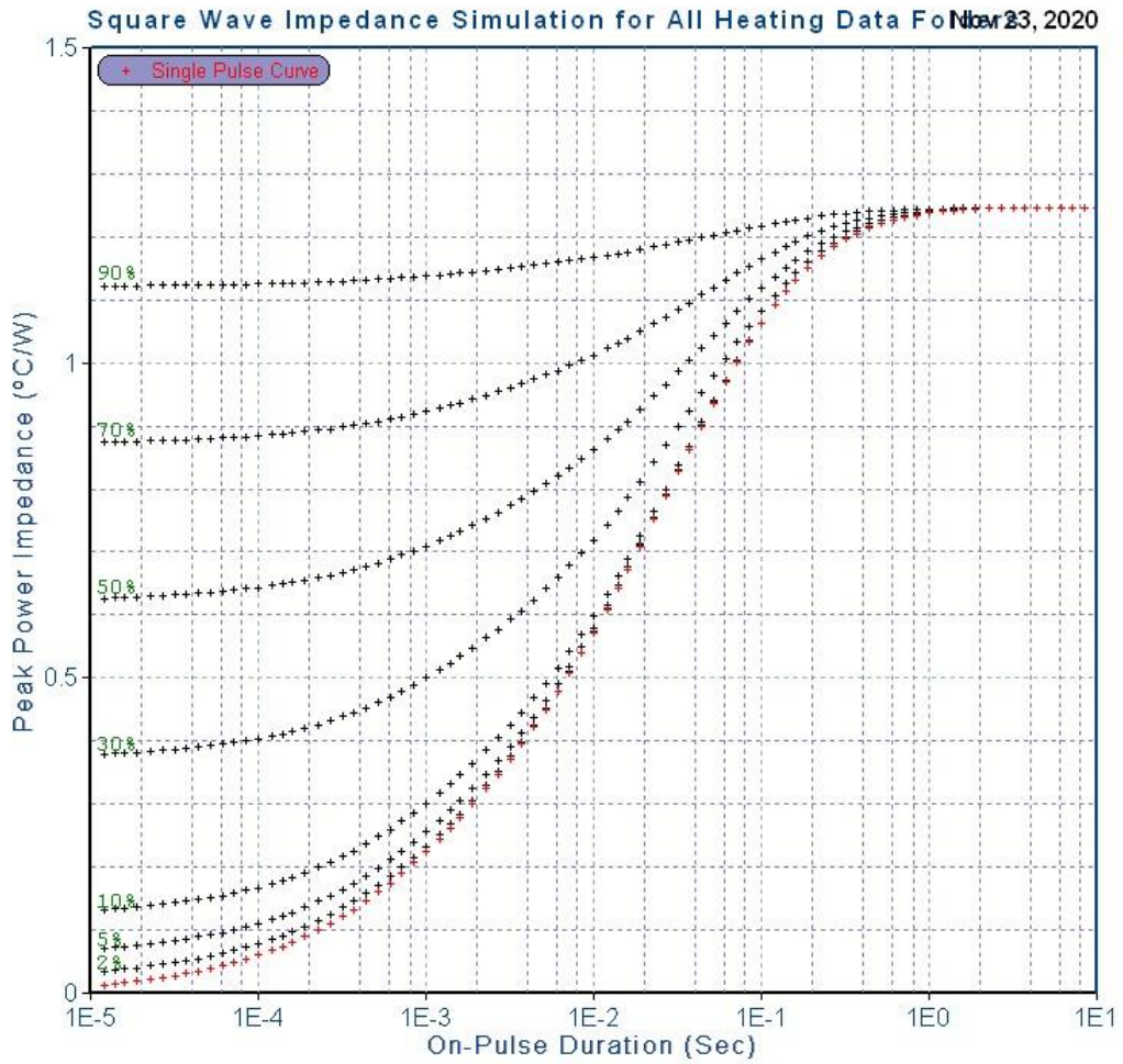
Transient Thermal Impedance of IGBT
