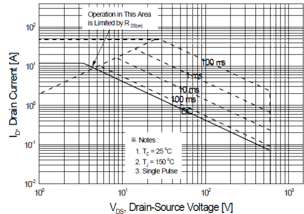
Figure 9-2. Maximum Safe Operating Area for JFFC13N65C
