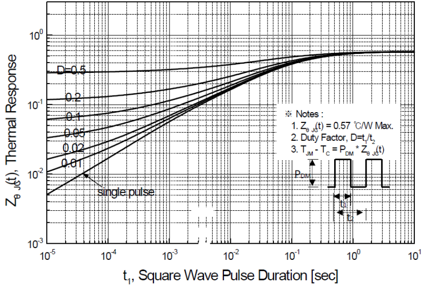
Figure 11-1. Transient Thermal Response Curve for JFPC13N65C
