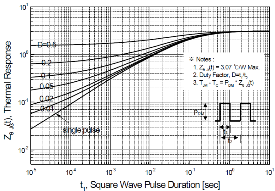
Figure 11-2. Transient Thermal Response Curve for JFFC13N65C
