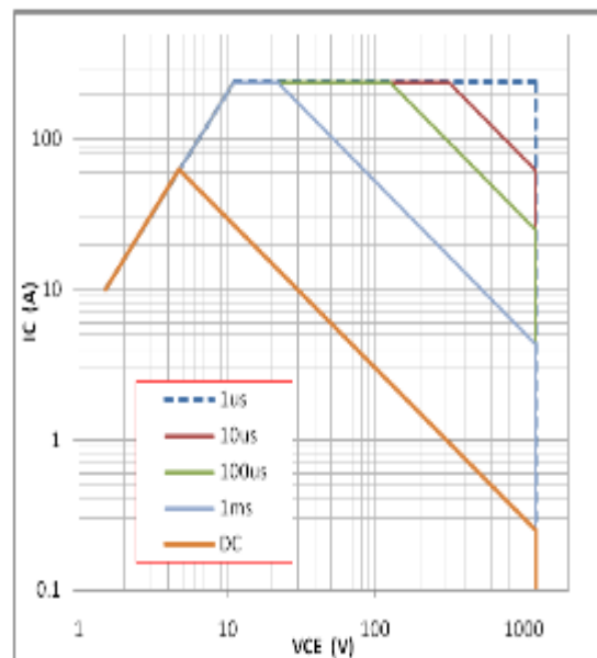
Figure4:forward SOA,TC=25°C,TJ≤150°C
