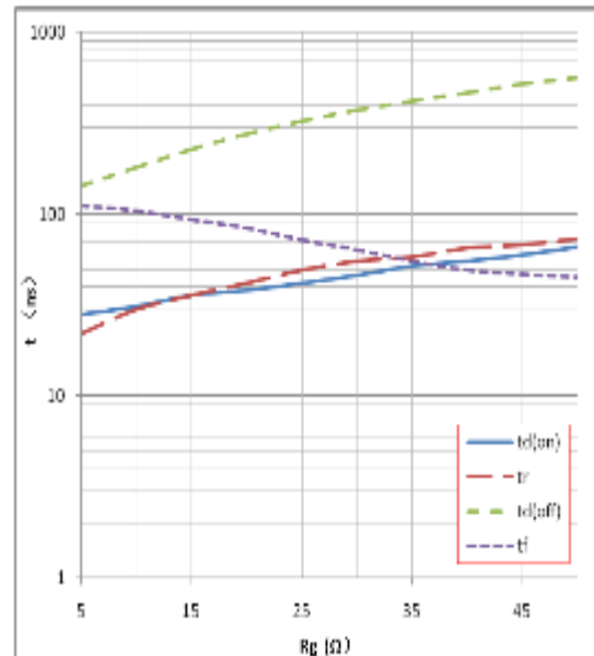
Figure12: typical switching time VS. Rg, TC=25°C, L=500uH, VCE=600V, VGE=15V, IC=20A
